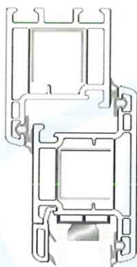
B-B Section
