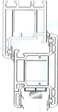
B-B Section
